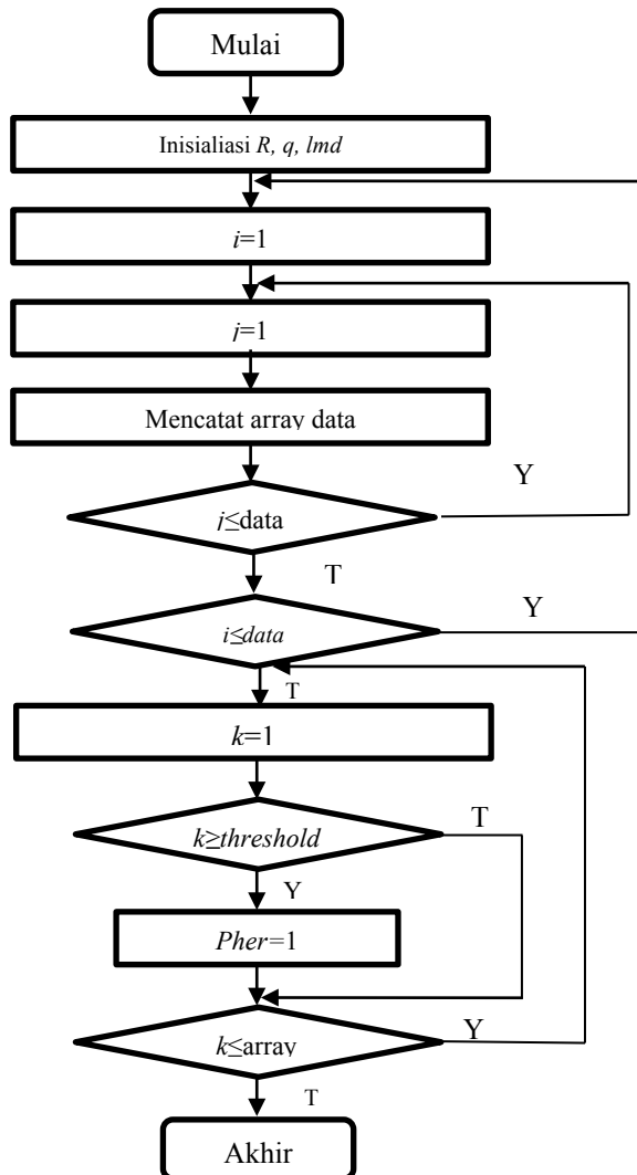
Gbr. 1 Algoritme Pattern Reduction.
