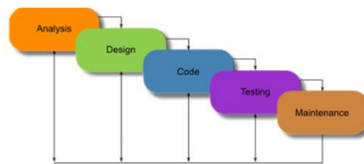
Gambar 1. Waterfall Model
