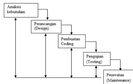
Gambar 2.1. Metode Waterfall
