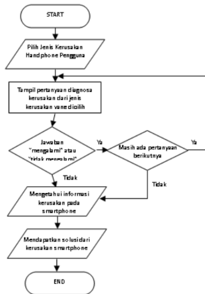
Gambar 3.4. Flowchart Proses Diagnosa
