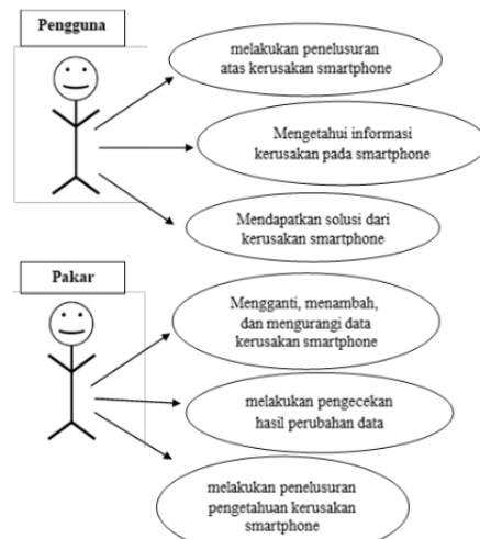
Gambar 2.3. Use Case
