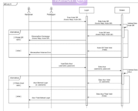
Figure 2 Sequence Diagram Log In
