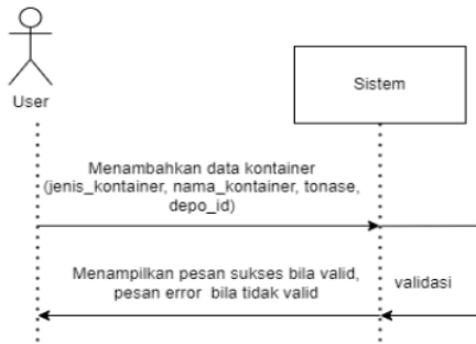
Gambar 4. Sequence Diagram Tambah Kontainer
