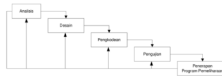
Gambar 1. Metode Waterfall
