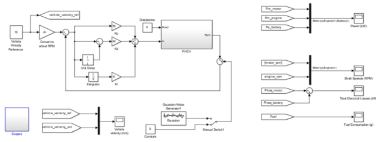
Figure 5. PID-HEV
