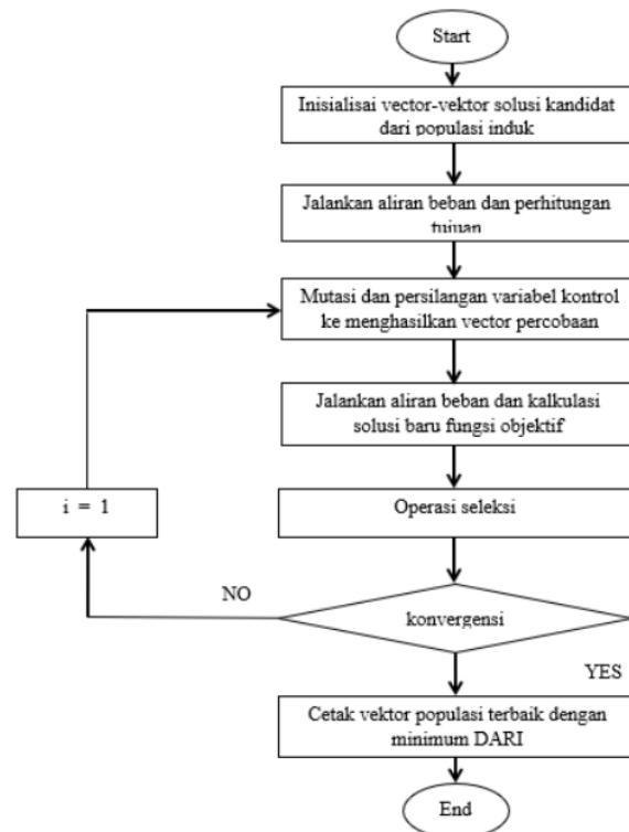
Figure 2. DE Algorithm Flowchat
