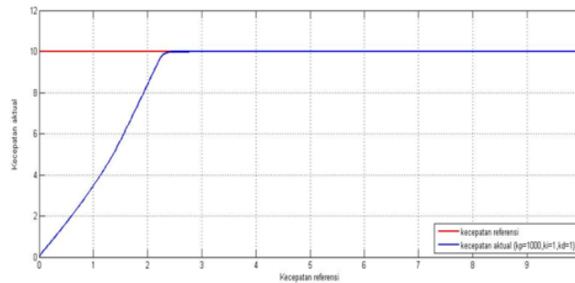
Figure 6. Graph of DE-1 Test Results
