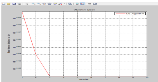
Figure 14. Graphic of BA-4 Test Results
