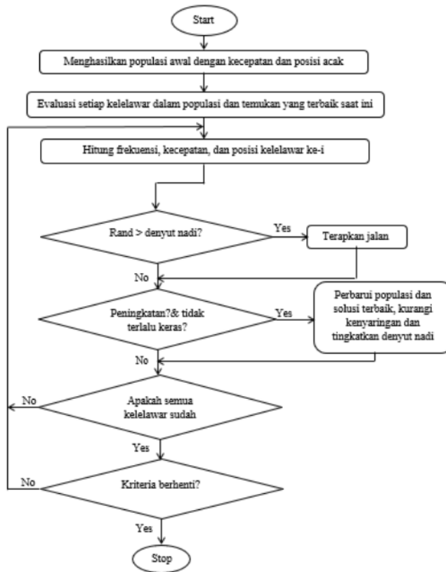
Figure 3. BA Algorithm Flowchat
