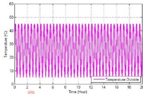
Fig. 5. Outside Temperature Air Model IV
