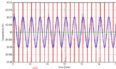
Fig. 16. Test IV Result with PID-DOB
