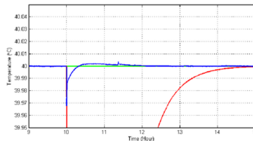
Fig. 14. Test III Result with PID-DOB
