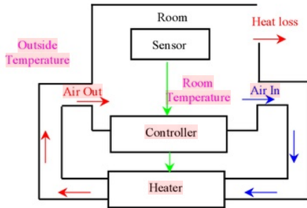
Fig. 1. Room Heating System
