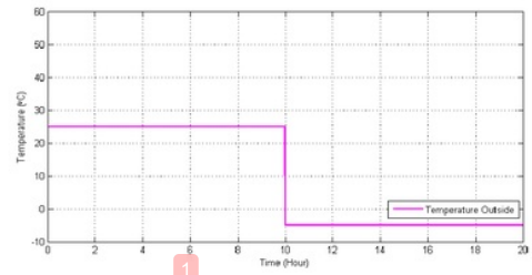
Fig. 4. Outside Temperature Air Model II
