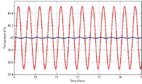
Fig. 15. Test IV Result with PID
