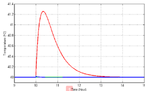
Fig. 11. Test II Result with PID
