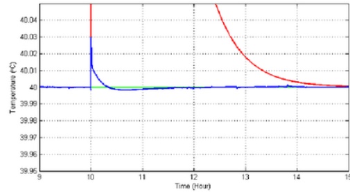
Fig. 12. Test III Result with PID-DOB
