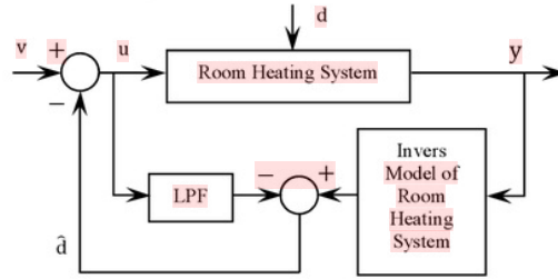
Fig. 6. Disturbance Observer
