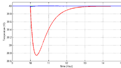
Fig. 13. Test III Result with PID
