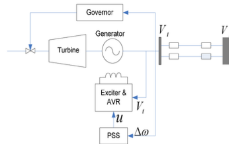
Figure 1. SMIB [4]
