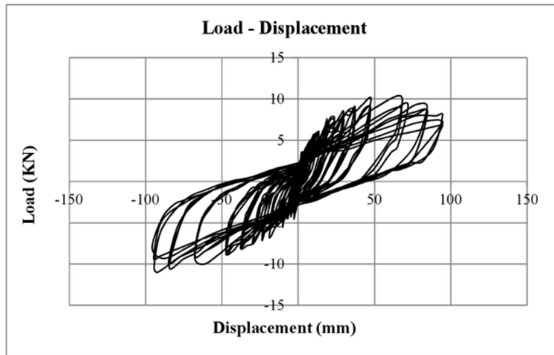
Figure 7. Hysteretic Curve Load-Displacement relationship specimen KP 1
