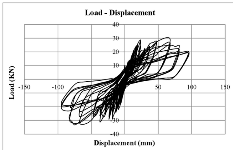
Figure 8. Hysteretic Curve Load-Displacement relationship specimen KP 2
