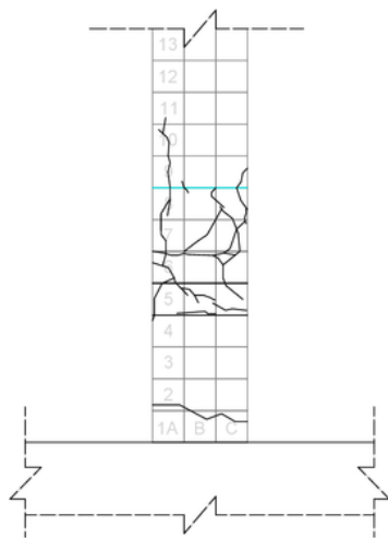
Figure 5. Crack pattern for KP 1
