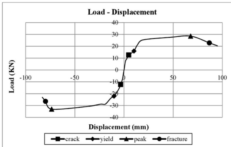
Figure 10. Envelope Curve Load-Displacement relationship specimen KP 2
