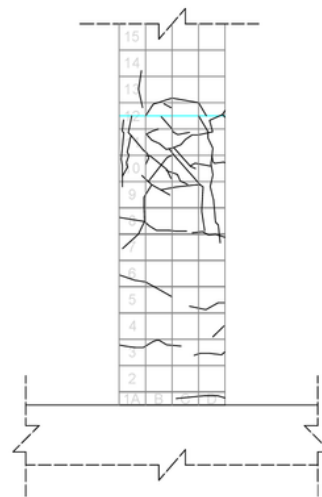
Figure 6. Crack pattern for KP 2
