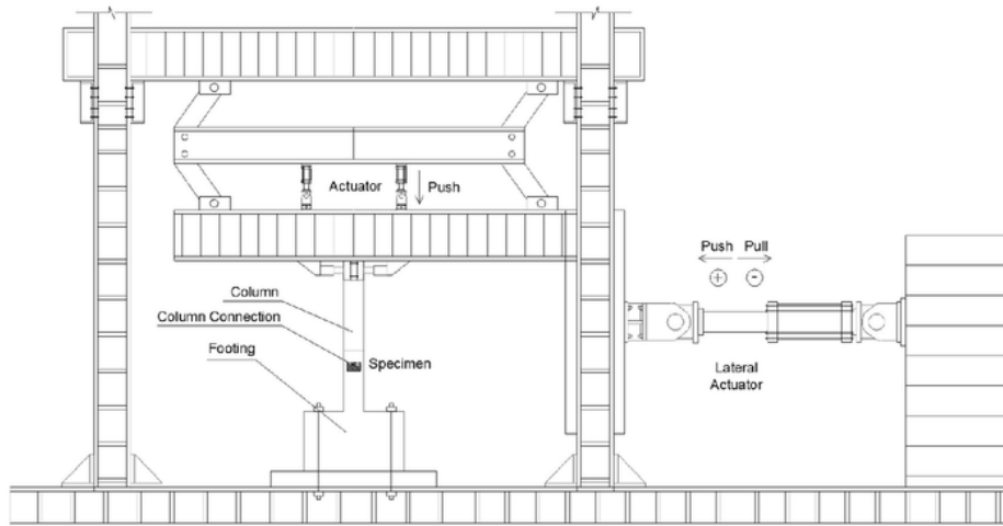
Figure 1. Test Setup for Experimental Study
