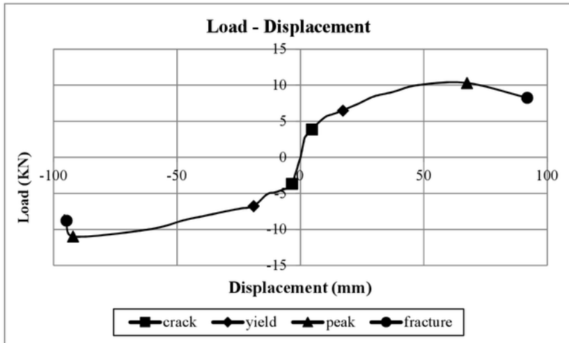
Figure 9. Envelope Curve Load-Displacement relationship specimen KP 1
