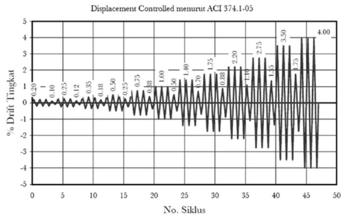
Figure 2. Cyclic Loading
