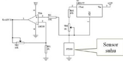
Gambar 7. Rangkaian Driver Sensor Suhu
