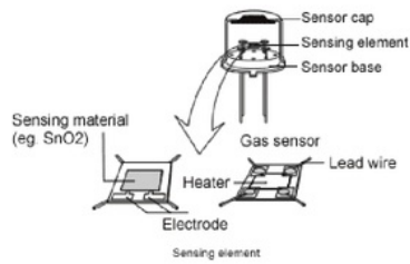
Fig. 1 - Sensor structure
